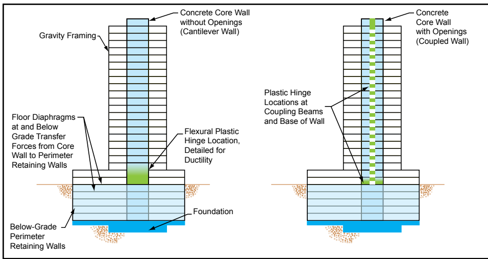
Figure 2: The typical nonlinear action for a cantilever wall (left) is a flexural plastic hinge at the base of the wall. For a coupled wall (right) nonlinear actions are flexure-yielding coupling beams and a flexural plastic hinge at the base of the wall.
