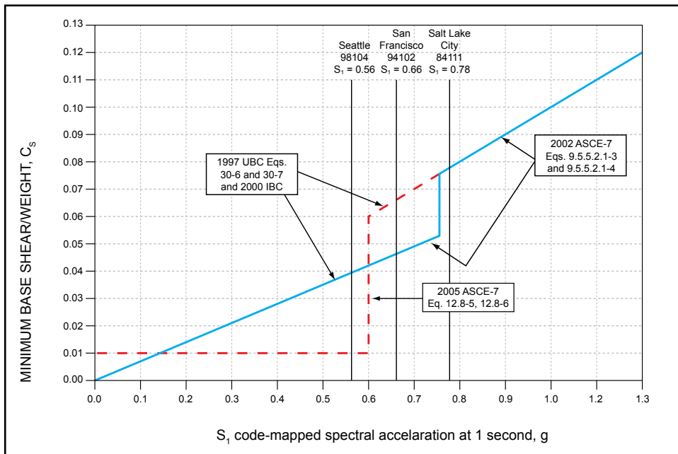
Figure 4: Minimum base shear equations for recent building codes, as a function of the ground motion parameter S_1 .
